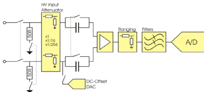
Front-end block diagram of a PXIe-2105 channel
